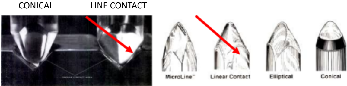
VIEW OF CONICAL AND LINE CONTACT STYLI AND GROOVE-TRACKING DIFFERENCES
