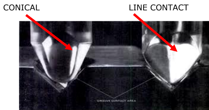
VIEW OF CONICAL AND LINE CONTACT STYLI AND WHY ALIGNMENT MATTERS MORE WITH THE LINE CONTACT.
